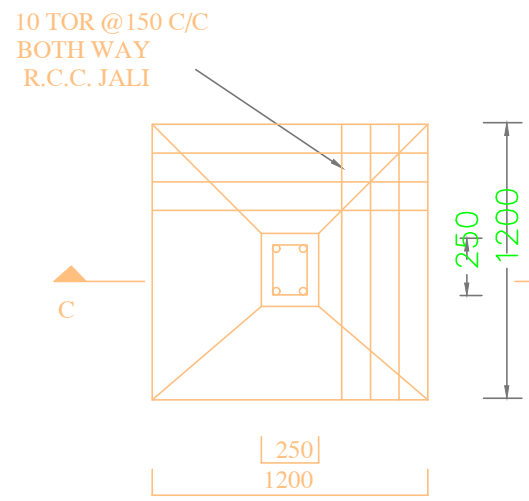
PLAN DETAIL OF FOUNDATION
