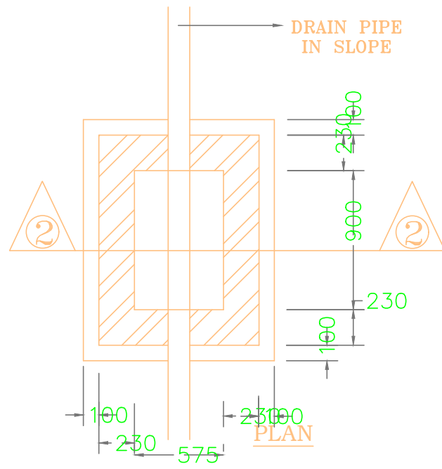
I.C. DETAILS
