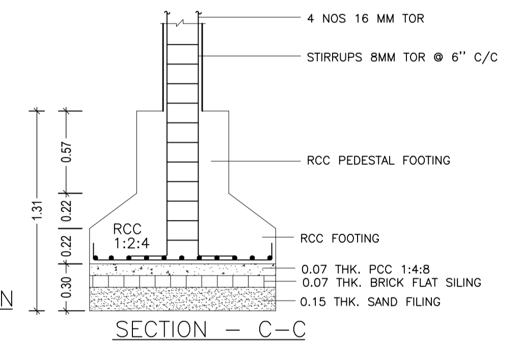
SECTION - C-C
