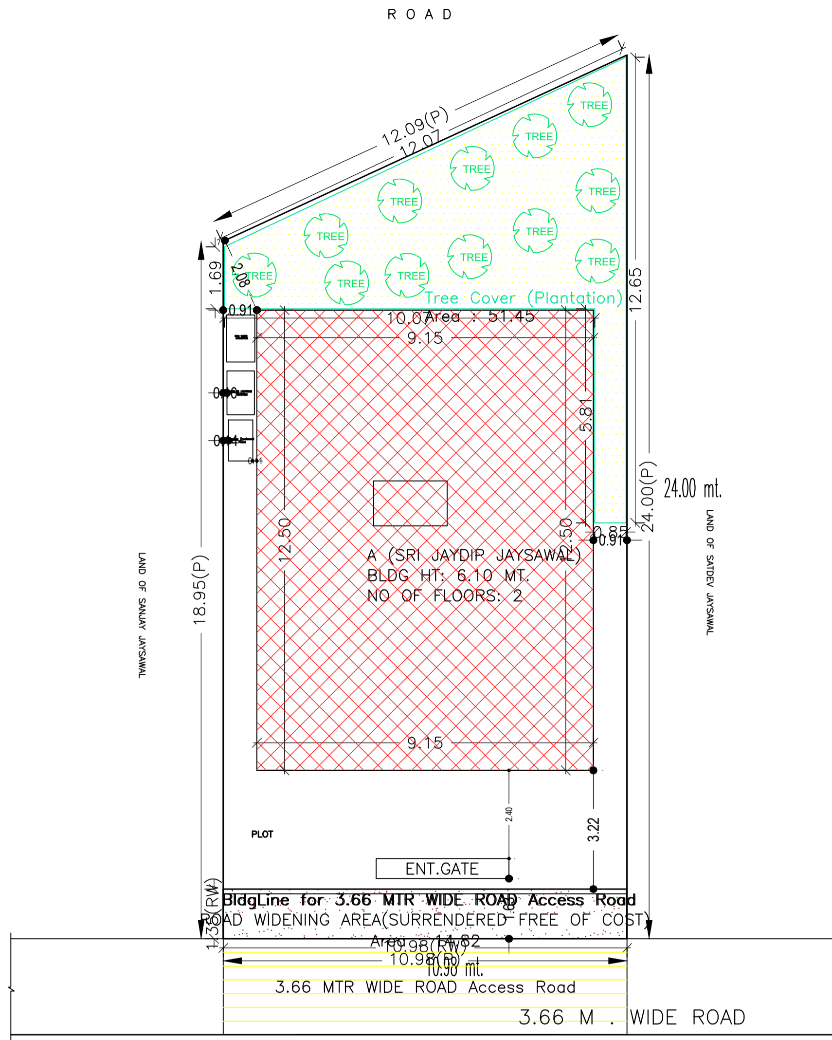
SITE PLAN
