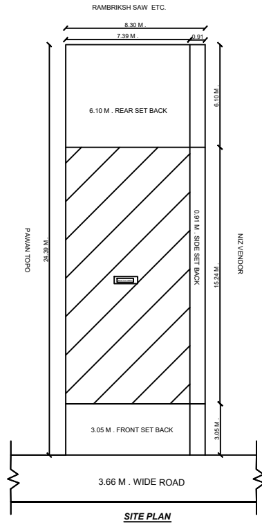
SITE PLAN
