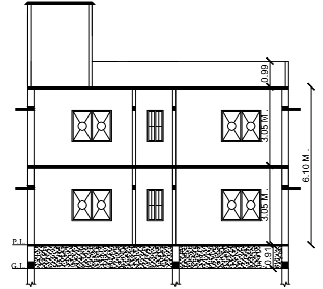
SECTION- XX
