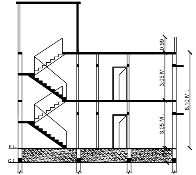
SECTION- YY
