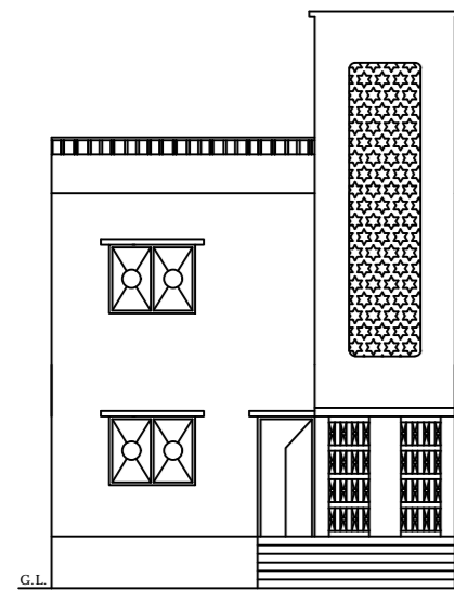
FRONT ELEVATION
