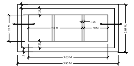
PLAN DETAIL OF SEPTIC TANK
