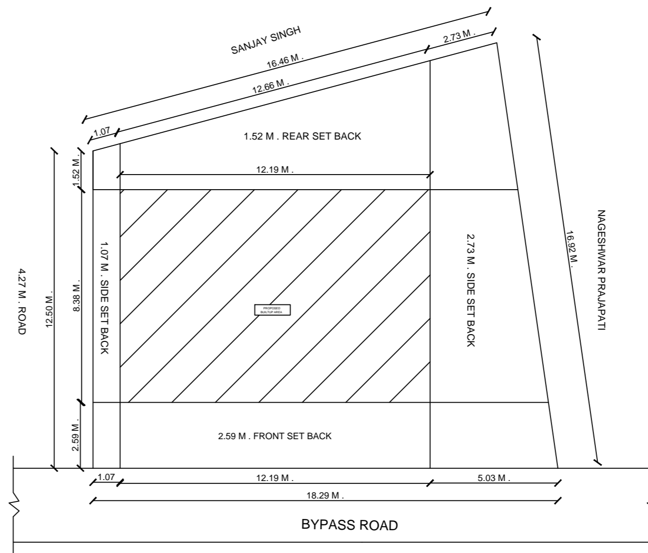
SITE PLAN
