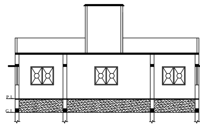
SECTION-YY
