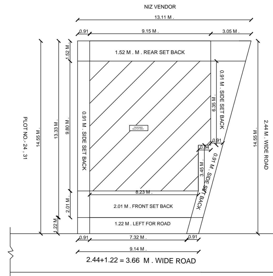
SITE PLAN
