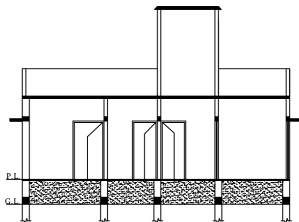
SECTION- XX
