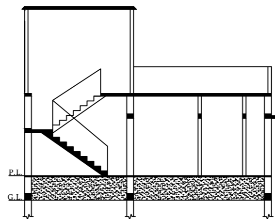
SECTION- YY
