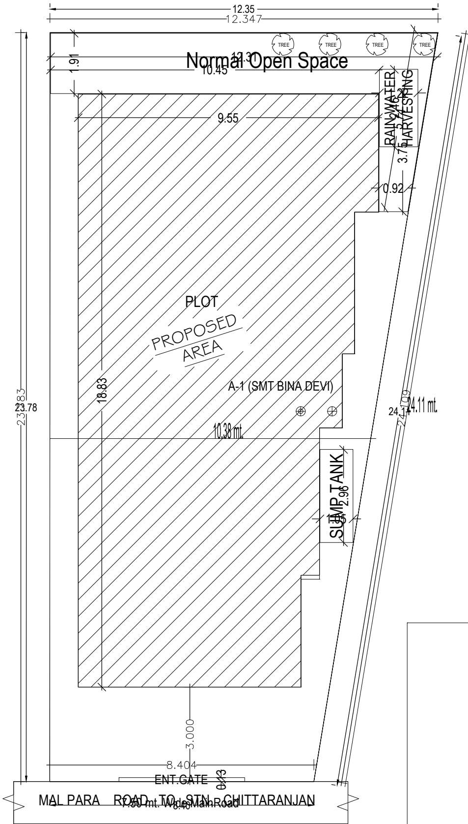
SITE PLAN
