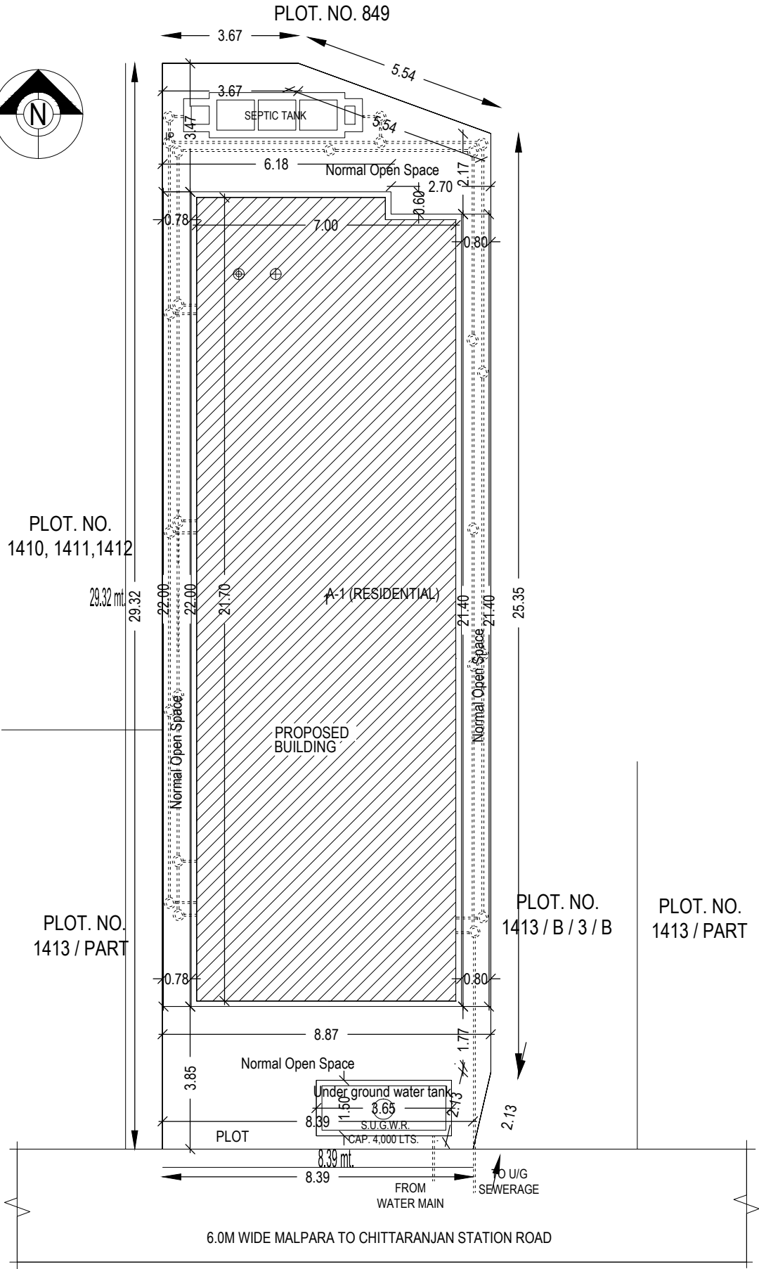
SITE PLAN
