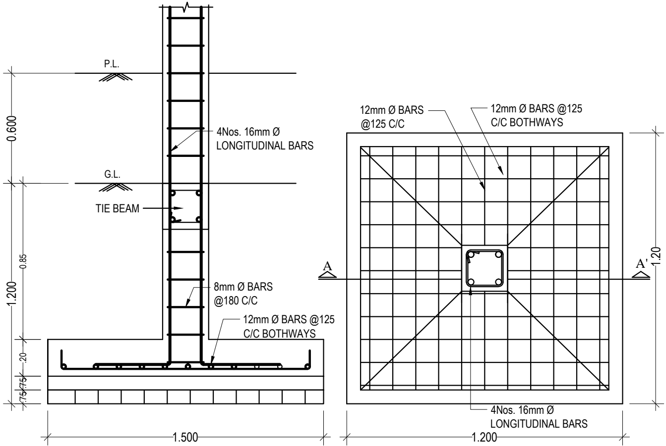
SECTION OF COLUMN(C1) (SCALE -1:25)
