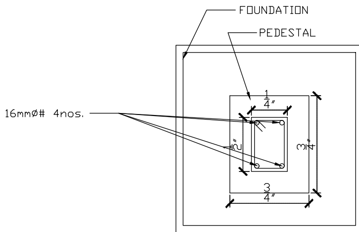
DETAIL OF FOOTING
