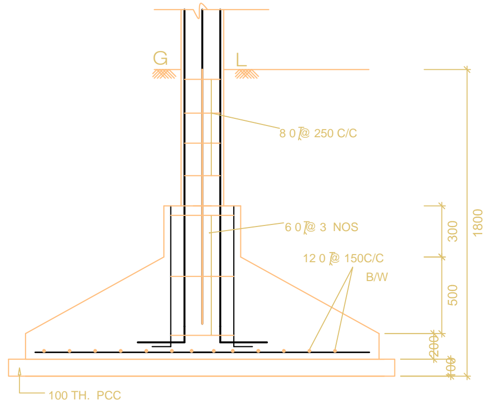
TYPICAL COLUMN FOUNDATION SCALE = 1:25
