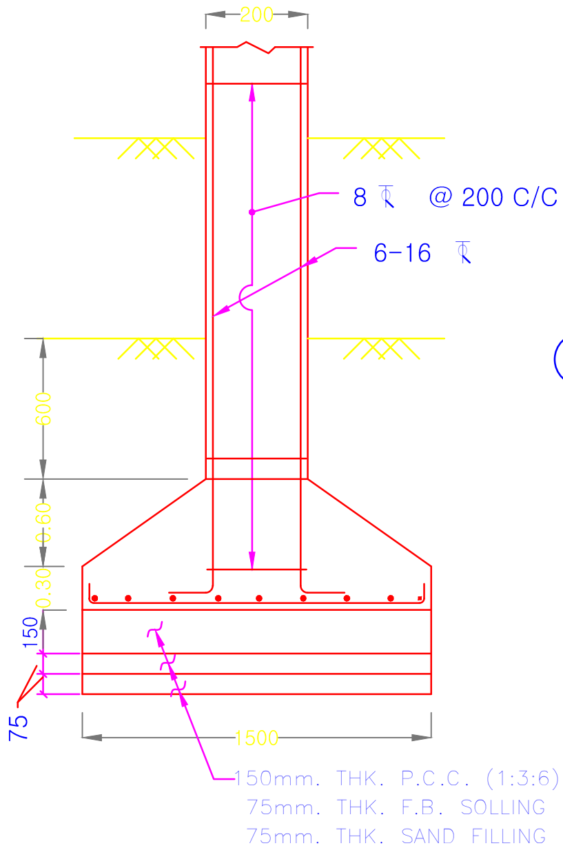
SECTION 4-4
