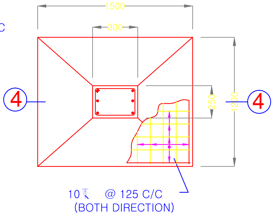
FOUNDATION PLAN OF COLUMN
