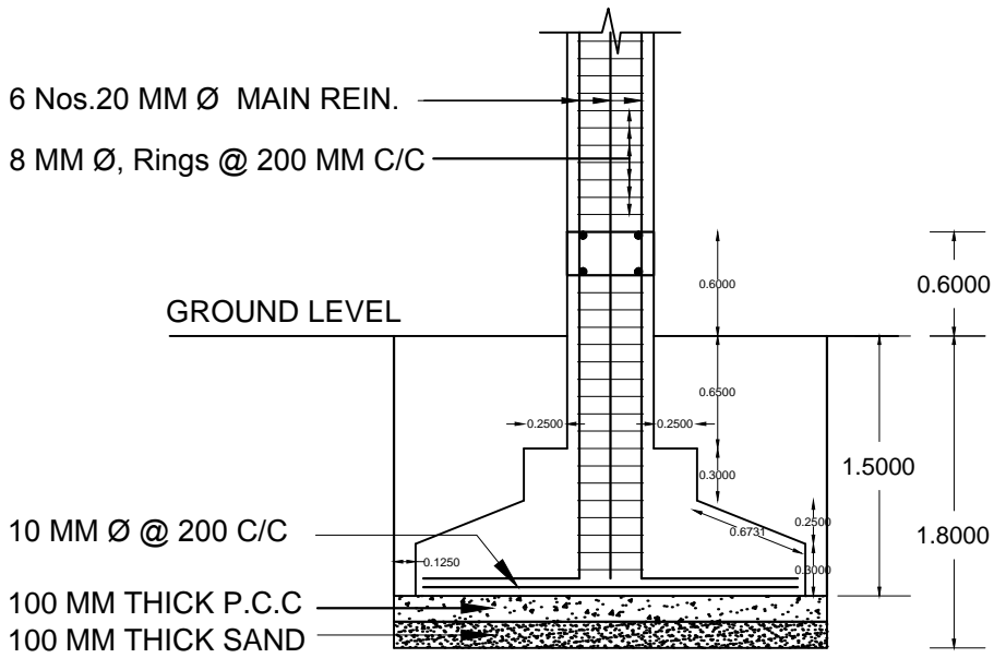
SECTION THROUGH FOUNDATION
