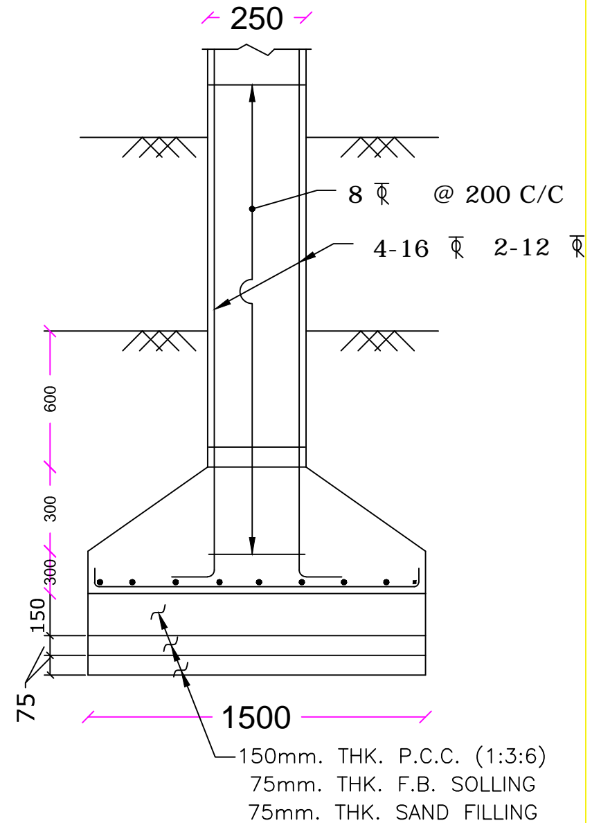
SECTION 4-4
