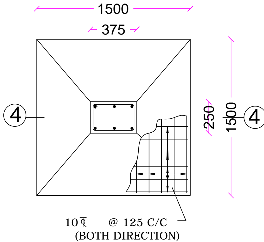
FOUNDATION PLAN OF COLUMN
