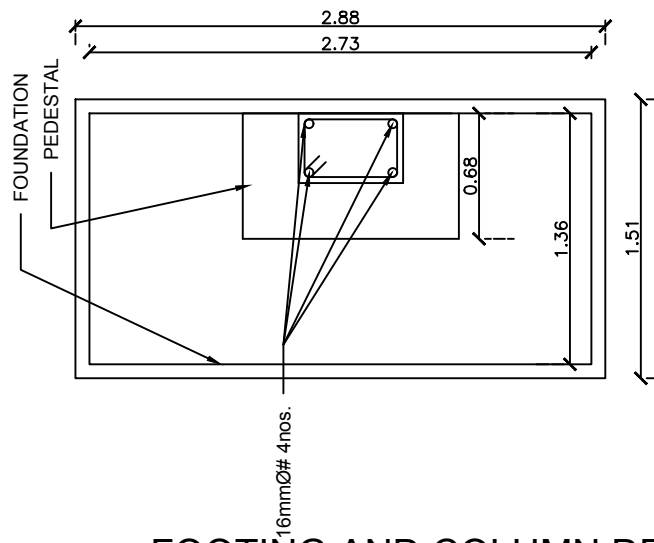
FOOTING AND COLUMN DETAIL
