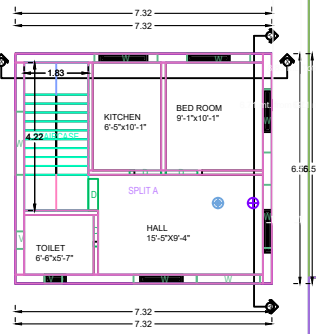
FIRST FLOOR PLAN (SCALE :- 1:100)
