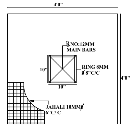
R.C.C. COLUMN FOOTING PLAN
