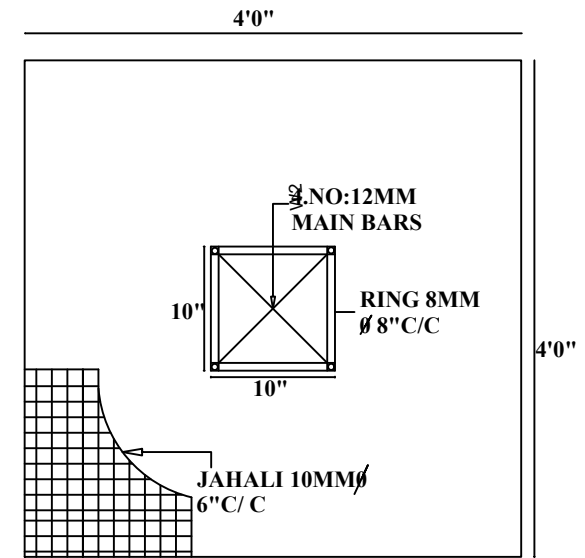
R.C.C.COLUMN FOOTING PLAN
