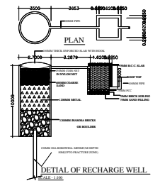
Sub Water Storage Tank Detail
