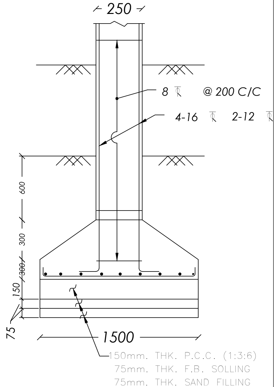
SECTION 4-4
