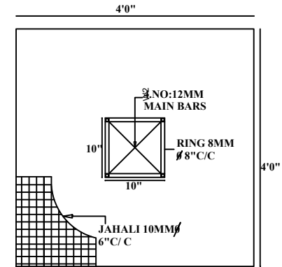
R.C.C.COLUMN FOOTING PLAN
