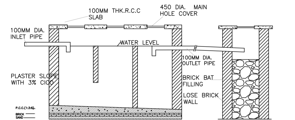
PLAN DETAIL OF SEPTIC TANK & SOAKPIT. SCALE - 1:50
