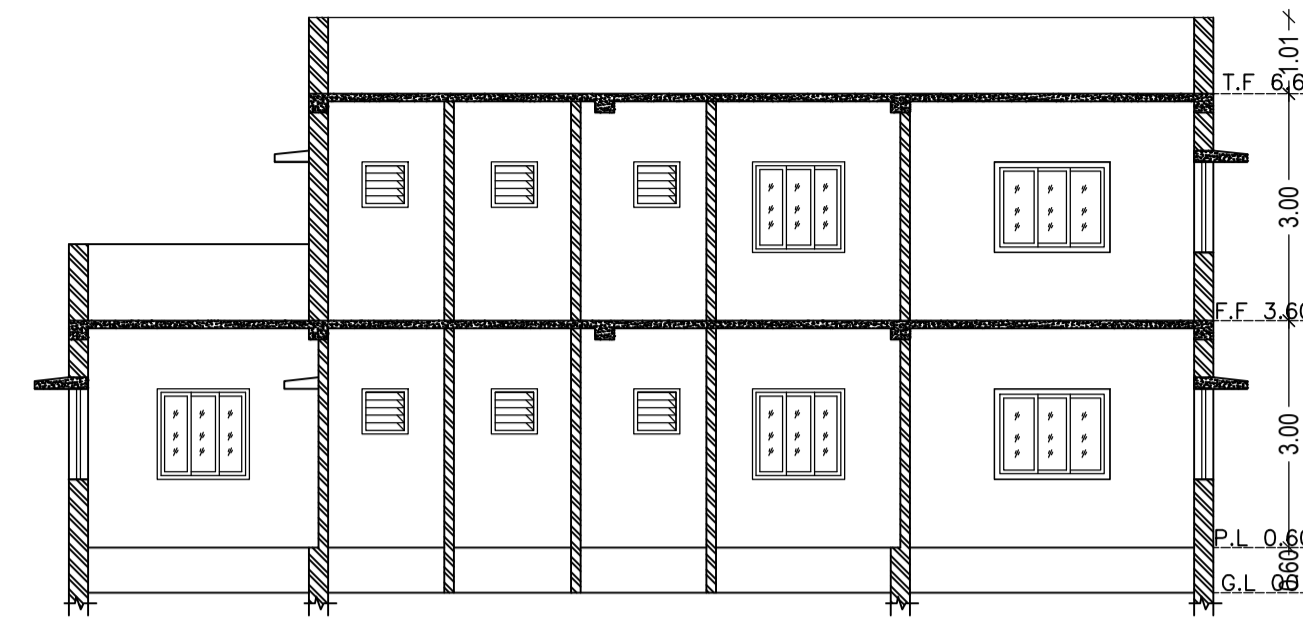
SECTION ON SCALE 1:100
