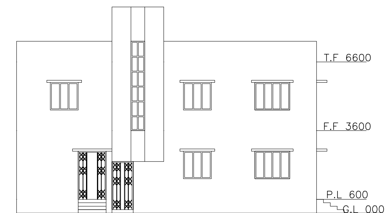
RIGHT SIDE ELEVATION SCALE 1:100
