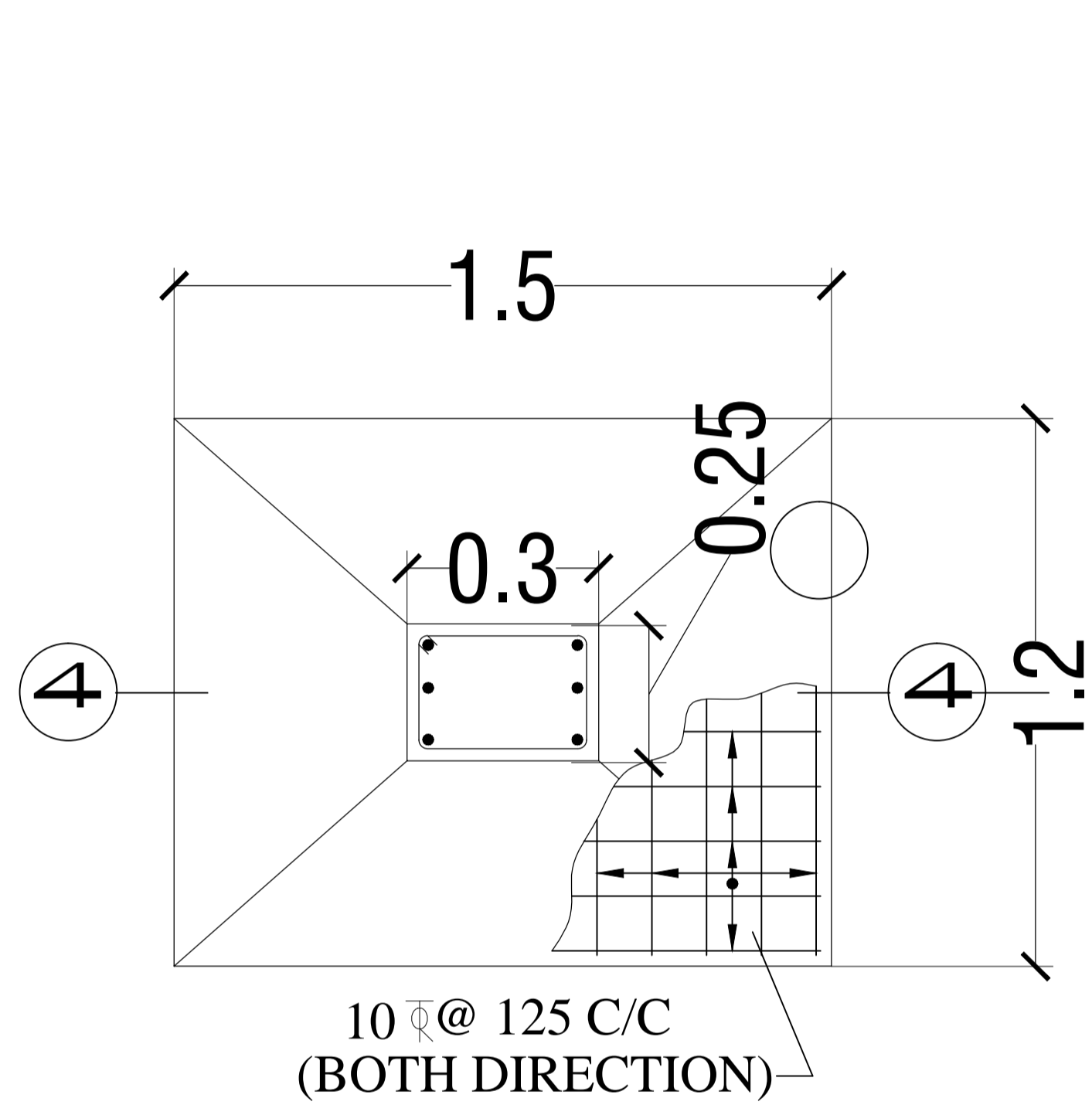
FOUNDATION PLAN OF COLUMN
