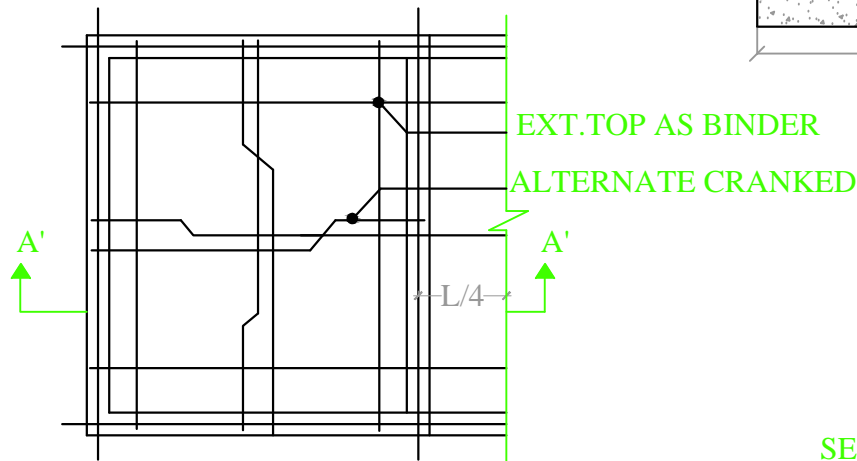
TYPICAL REINFORCEMENT DETAIL
