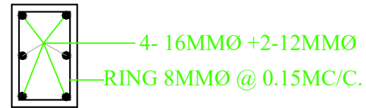
SECTION OF COLUMN.
