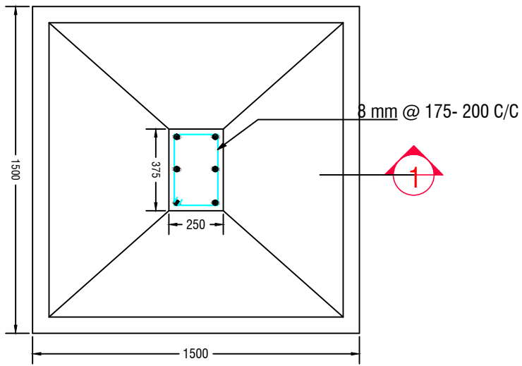
6 Nos.- 16 mm Dia Bar TYPICAL FOUNDATION SCALE -1:25
