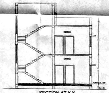
SECTION AT X X SCALE 1:100
