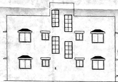
RIGHT SIDE ELEVATION SCALE 1:100
