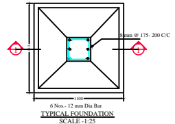
TYPICAL FOUNDATION SCALE-1:25
