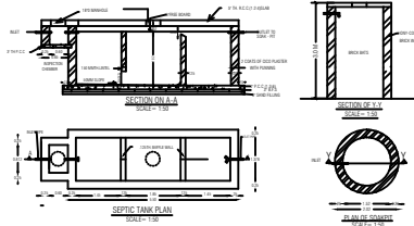
SEPTIC TANK PLAN SCALE-1:50
