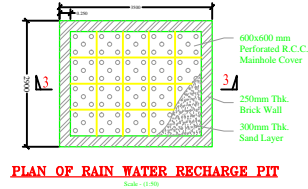
PLAN OF RAIN WATER RECHARGE PIT Scale-1:30
