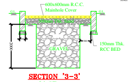
SECTION '3-3' Scale-1:30
