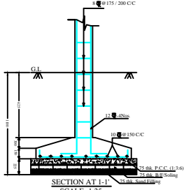
SECTION AT 1-1' SCALE - 1:25
