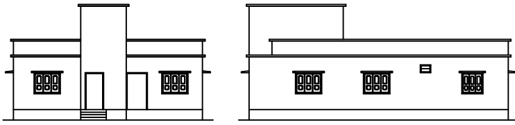
FRONT ELEVATION 1:100
