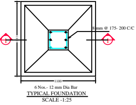
TYPICAL FOUNDATION SCALE - 1:25
