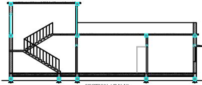
SECTION AT Y-Y' 1:100
