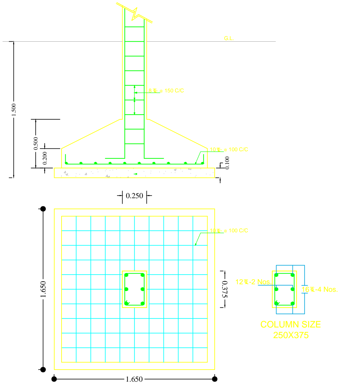
FOOTING DETAILS
