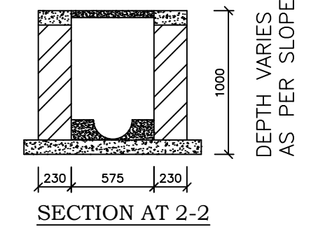
SECTION AT 2-2
