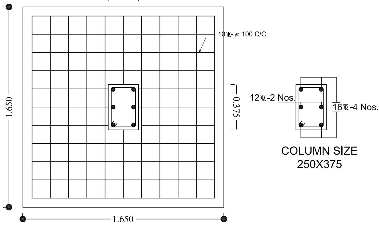
FOOTING DETAILS
