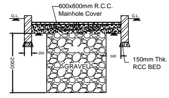
SECTION '3-3' Scale - (1:50)
