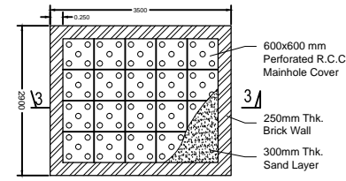
PLAN OF RAIN WATER RECHARGE PIT Scale - (1:50)
