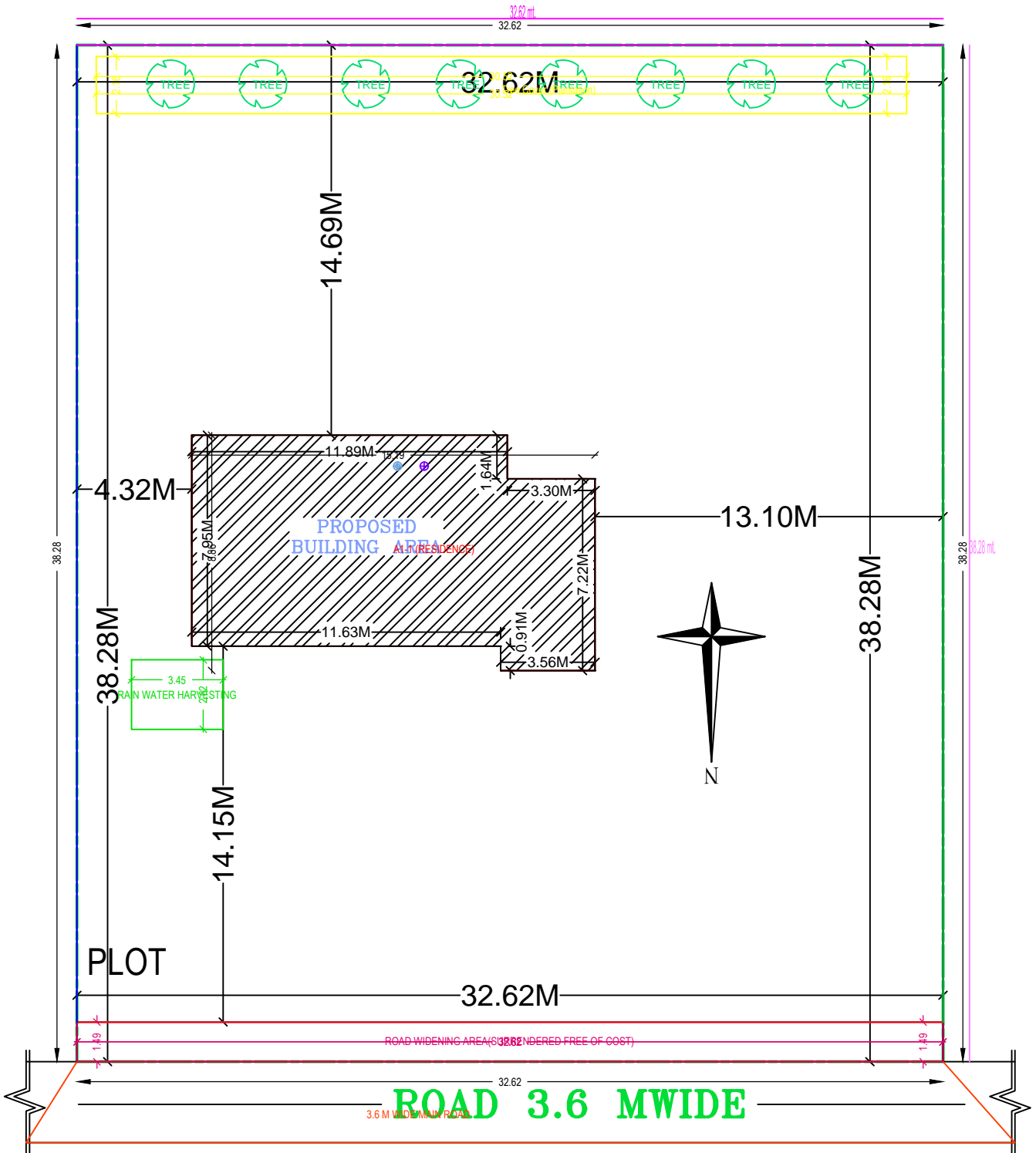
SITE PLAN
