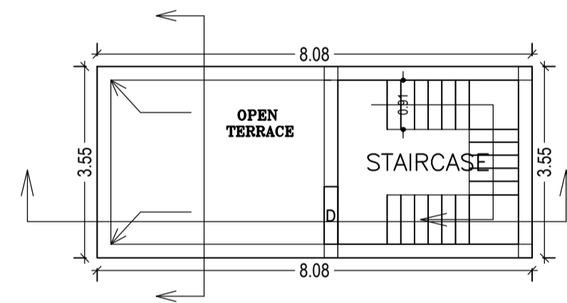
FIRST FLOOR PLAN (Proposed) (SCALE 1:100)
