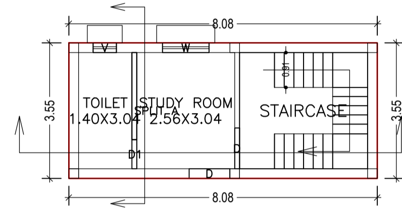
GROUND FLOOR PLAN (Proposed) (SCALE 1:100)
