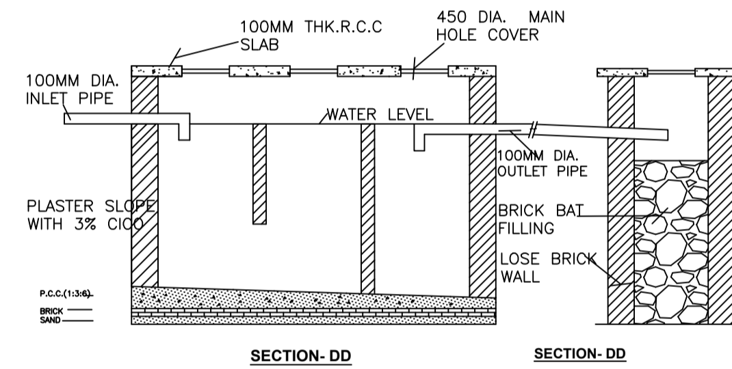
SECTION-DD
