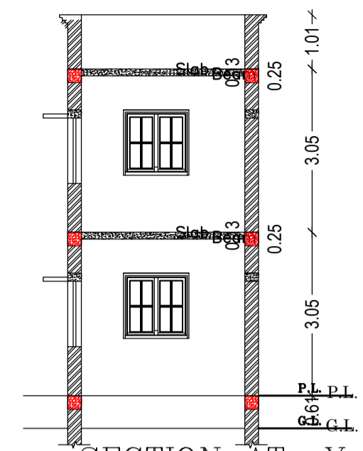
SECTION AT: Y-Y SCALE 1:100
