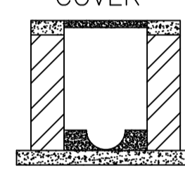
SECTION AT 2-2
