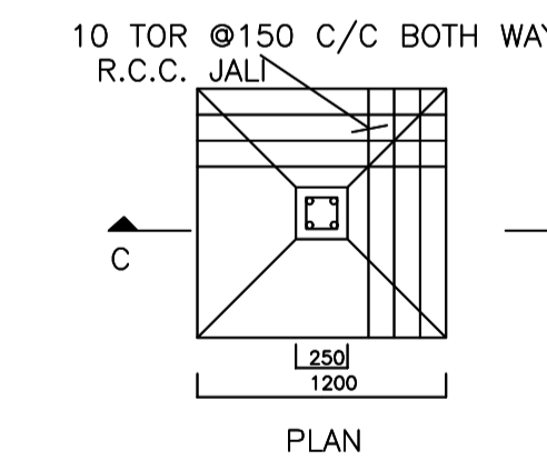
DETAIL OF FOUNDATION SCALE:- 1:50
