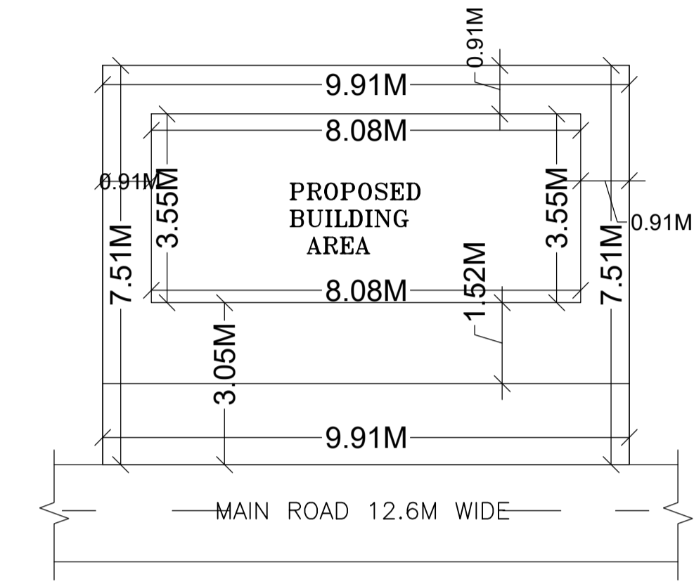
KEY PLAN SCALE 1:100
