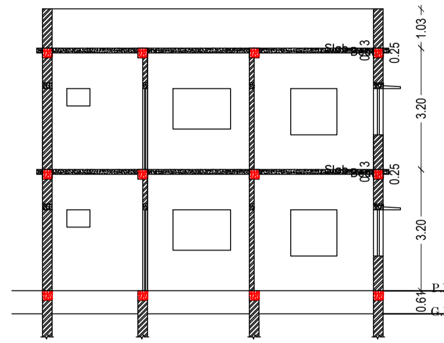
SECTION ON SCALE 1:100
