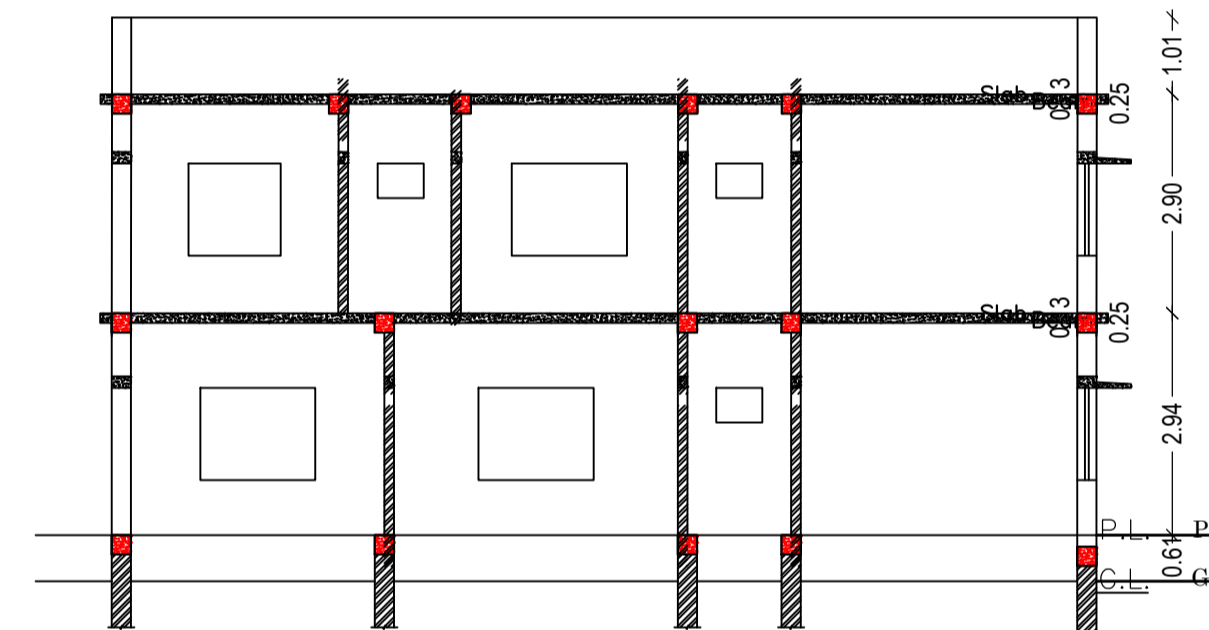
SECTION AT-Y-Y SCALE 1:100
