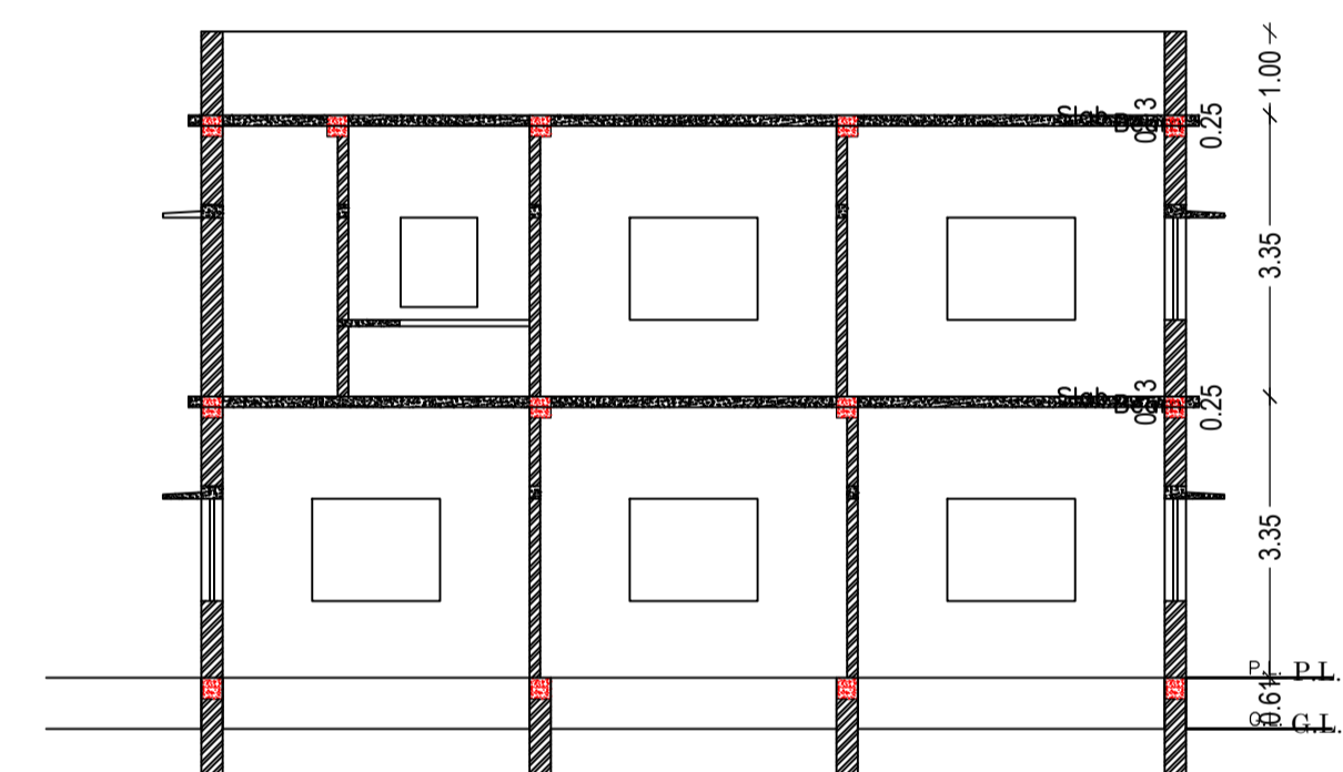
SECTION AT-Y-Y SCALE 1:100
