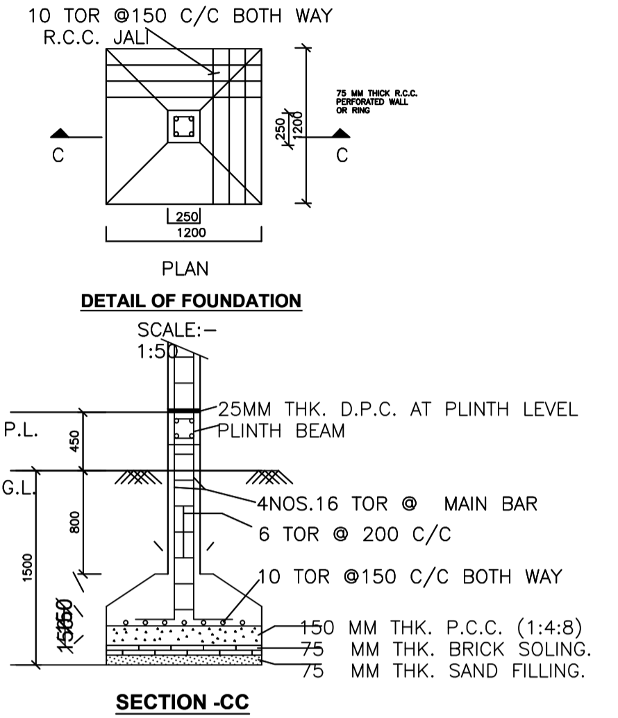
SECTION-CC
