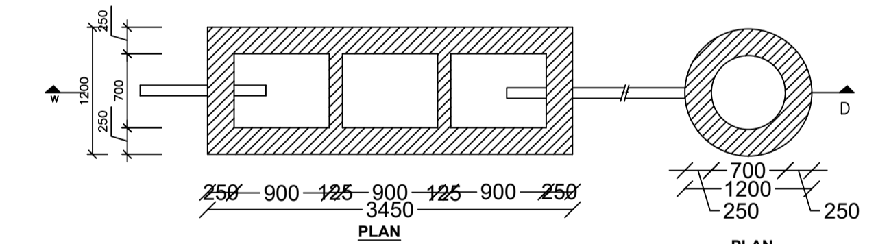
DETAIL OF SEPTIC TANK & SOAKPIT. PLAN SCALE - 1:50
