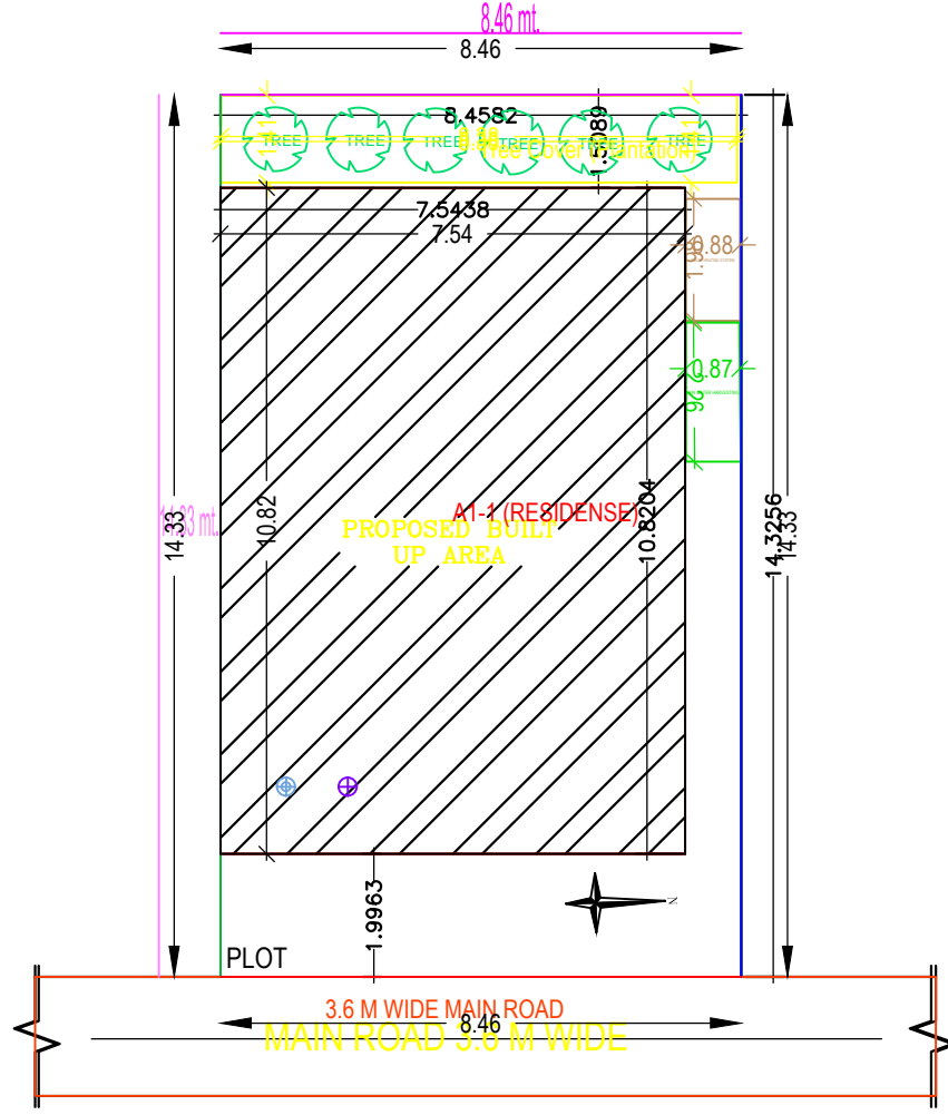
KEY PLAN SCALE 1:100
