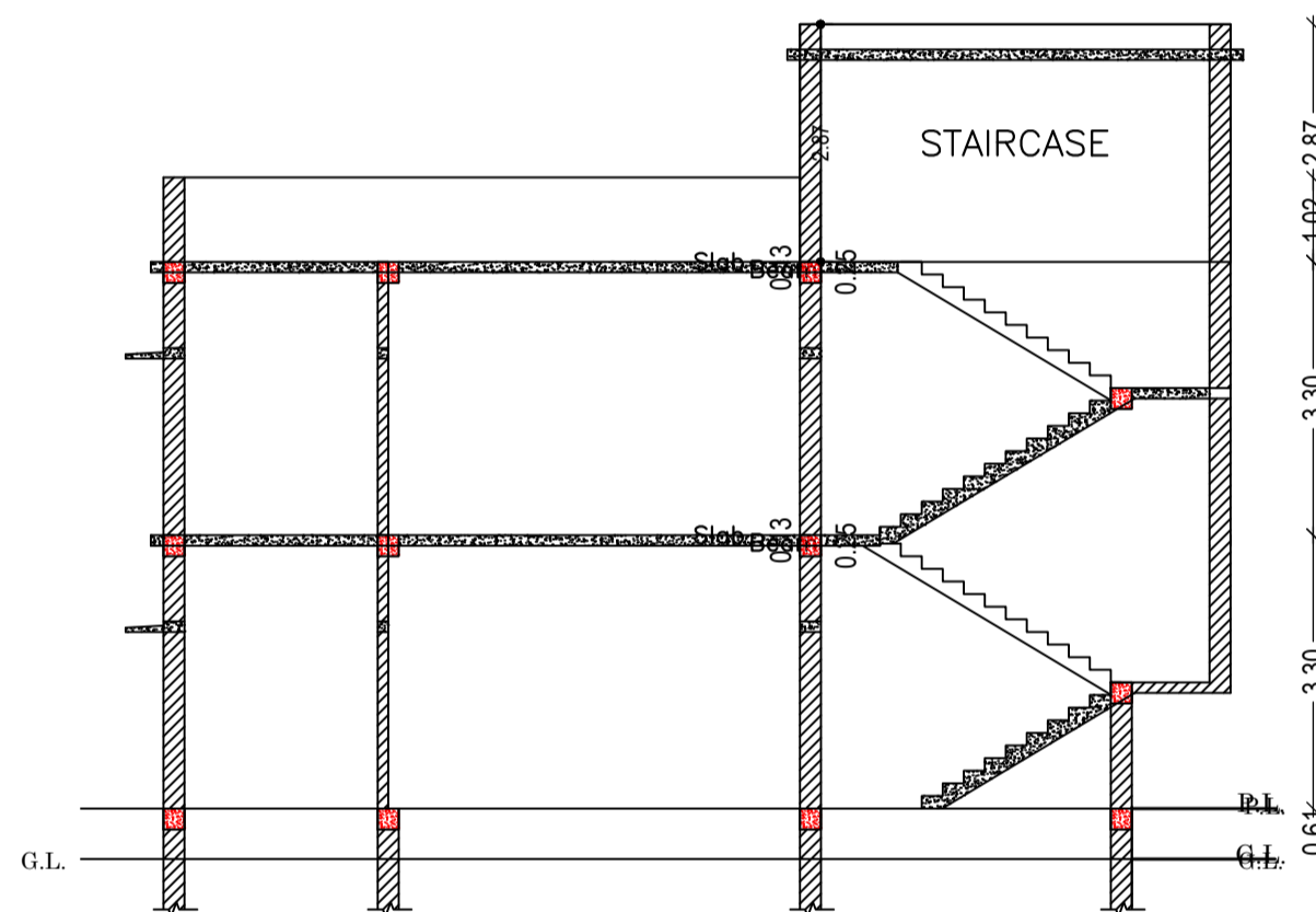
SECTION ON Y-Y (SCALE 1:100)
