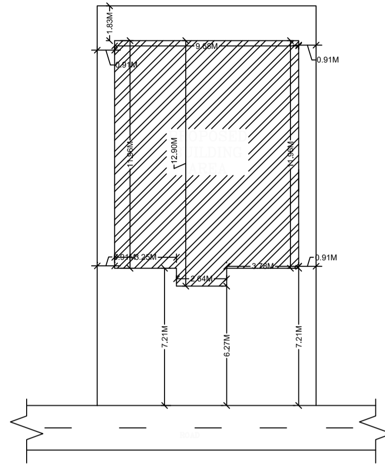
KEY PLAN (SCALE 1:200)
