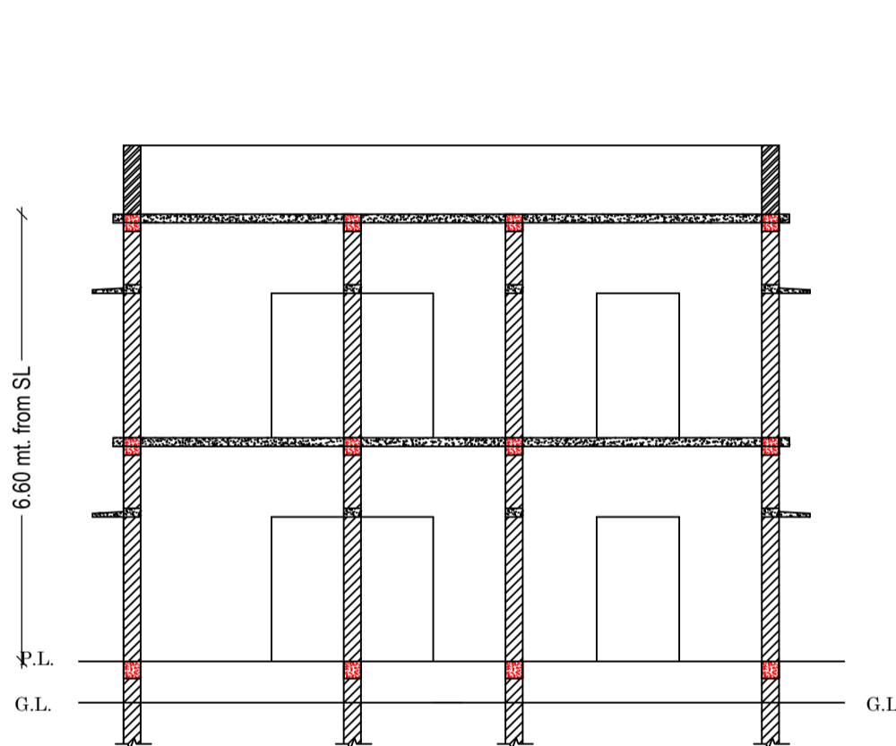
SECTION ON X-X (SCALE 1:100)
