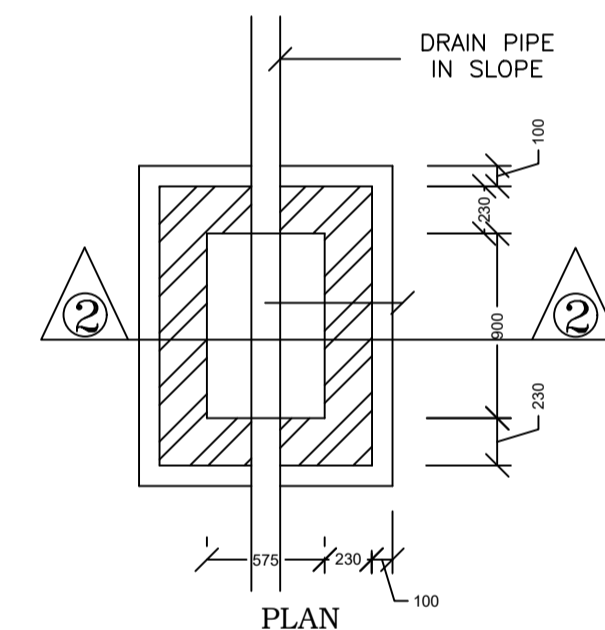
I.C. DETAILS (SCALE 1:50)
