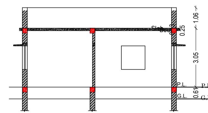
SECTION AT-Y-Y SCALE 1:100
