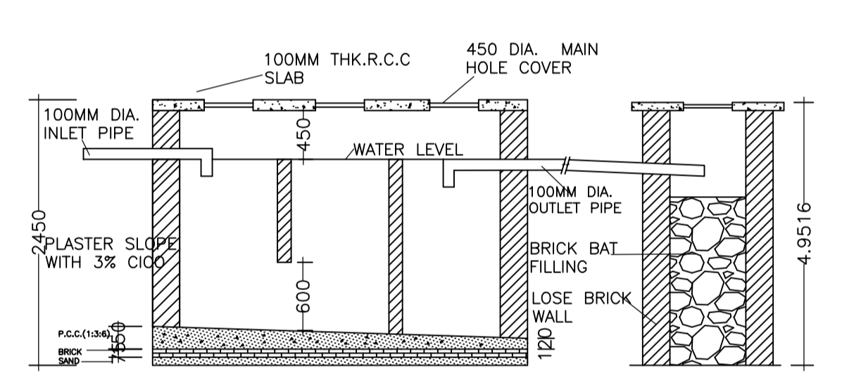
SECTION-DD
