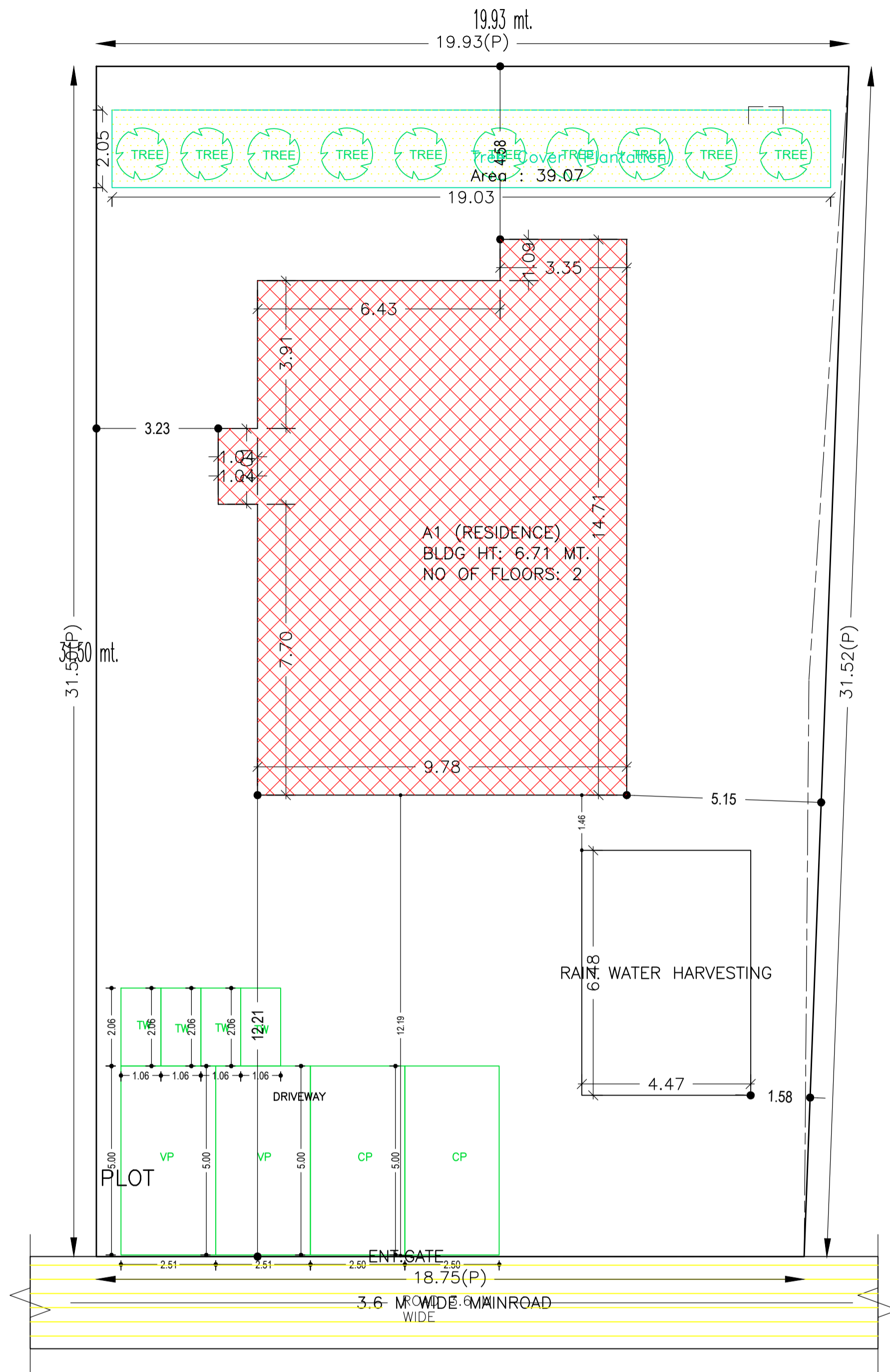
SITE PLAN
