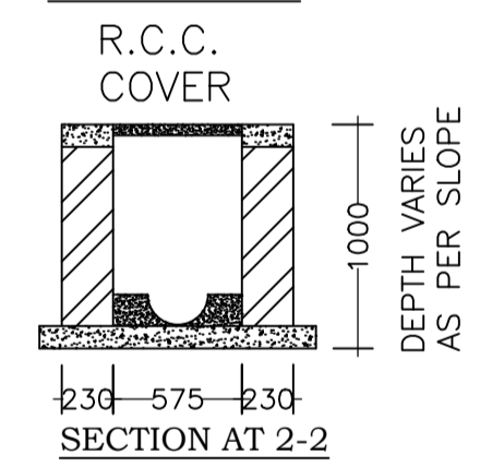
SECTION AT 2-2
