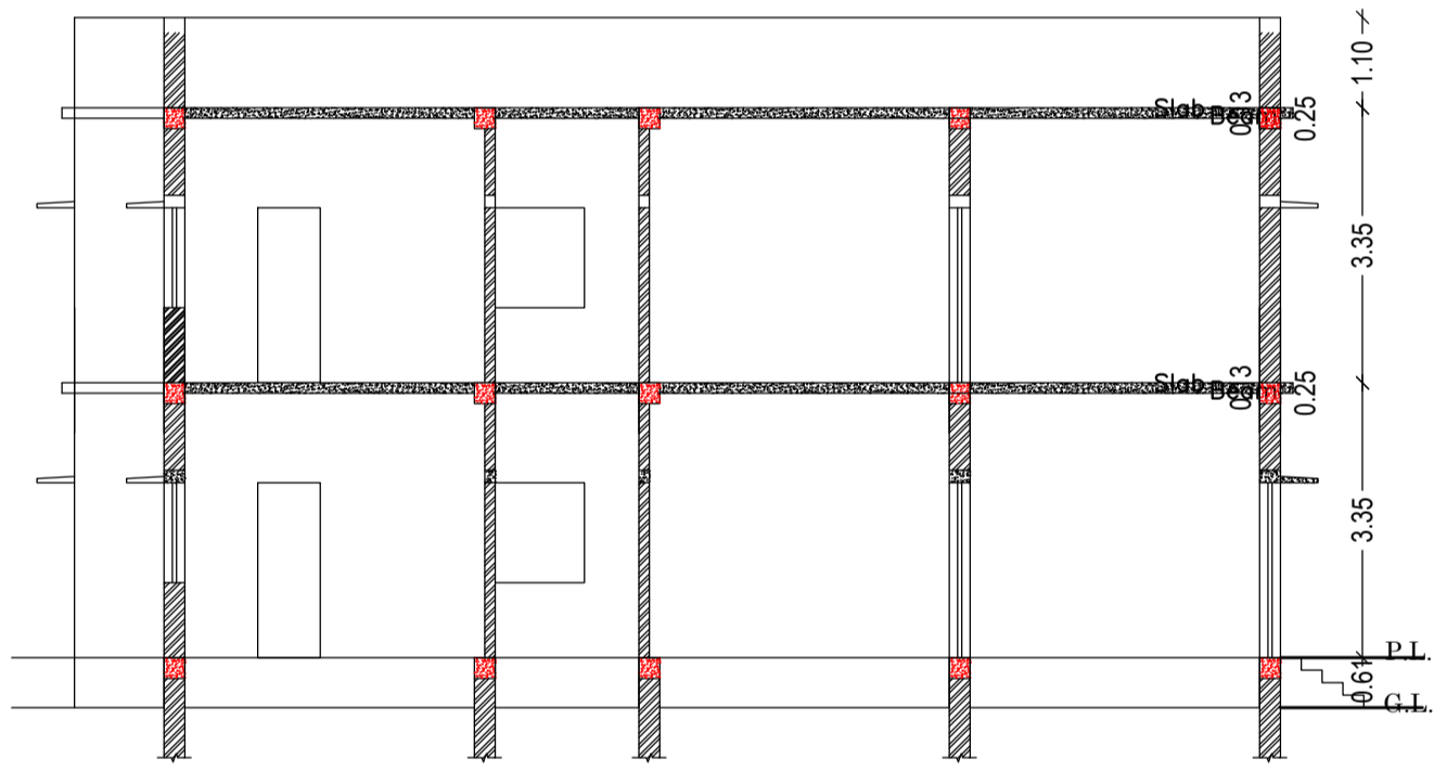
SECTION AT-Y-Y (SCALE 1:100)
