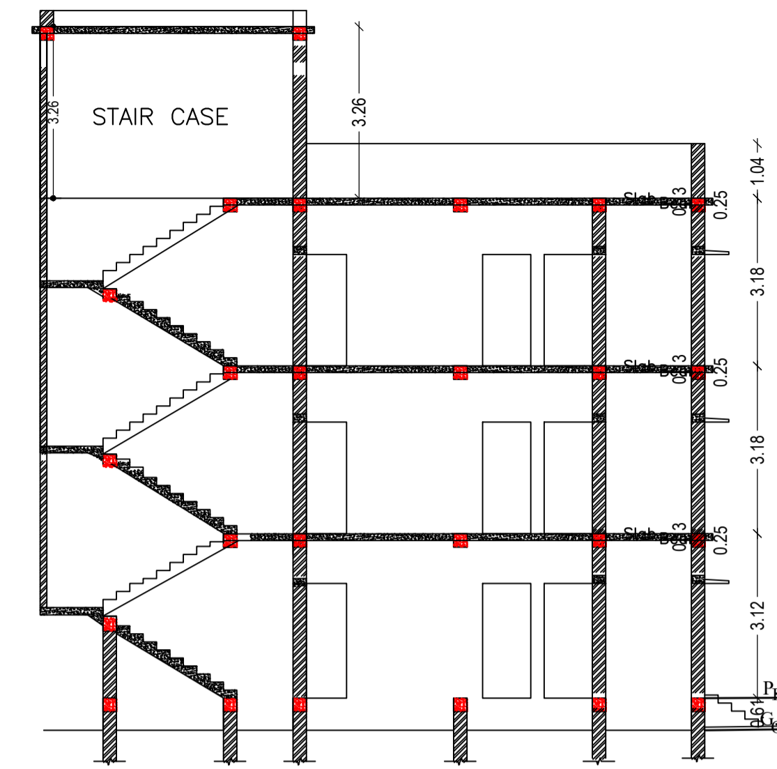
SECTION ON SCALE 1:100
