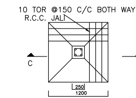
PLAN SCALE 1:50
