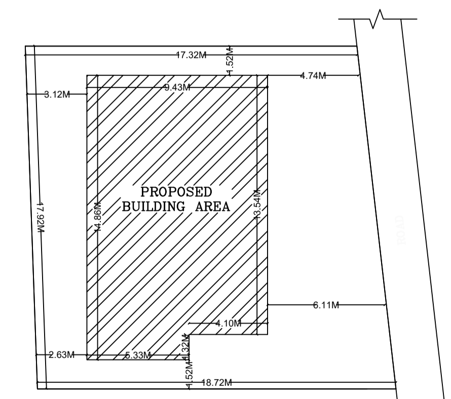
KEY PLAN (SCALE 1:200)
