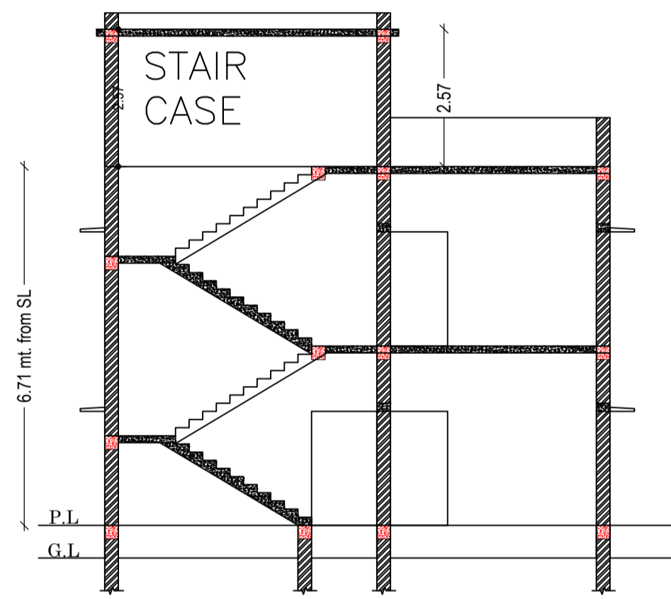
SECTION ON (SCALE 1:100)
