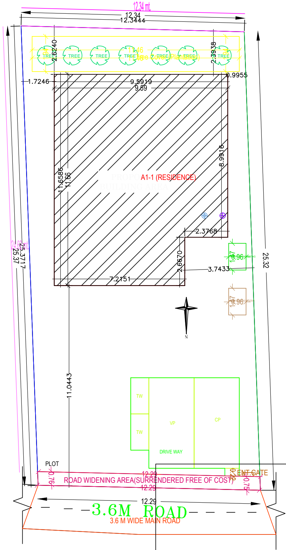
SITE PLAN
