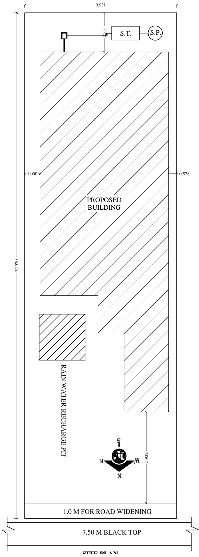
SITE PLAN
