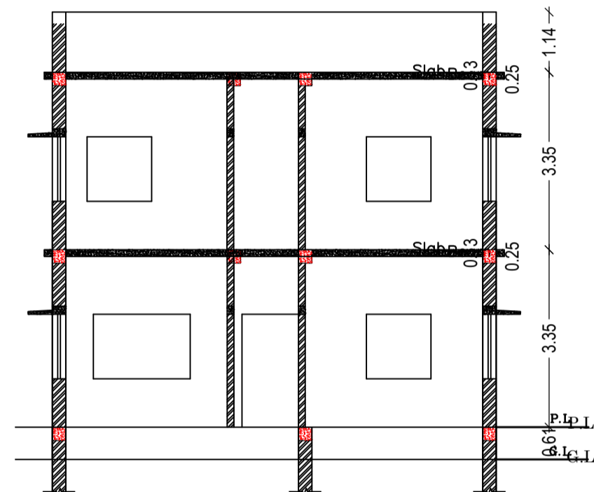
SECTION ON SCALE 1:100
