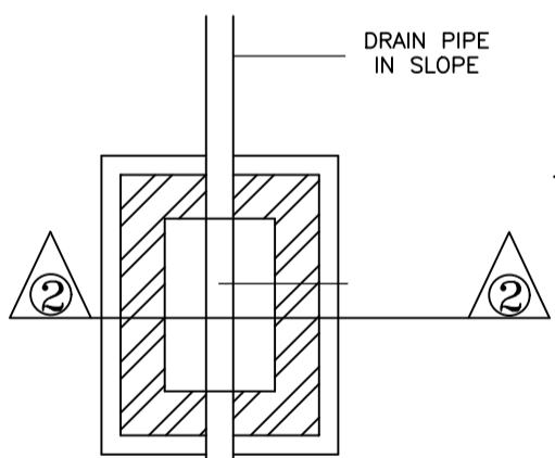
PLAN I.C.DETAILS R.C.C. COVER
