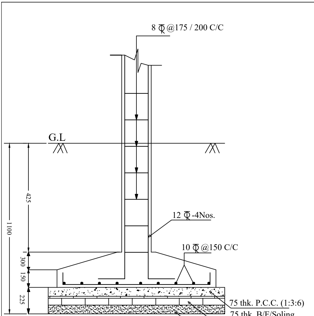
SECTION AT 1-1' SCALE -1:25
